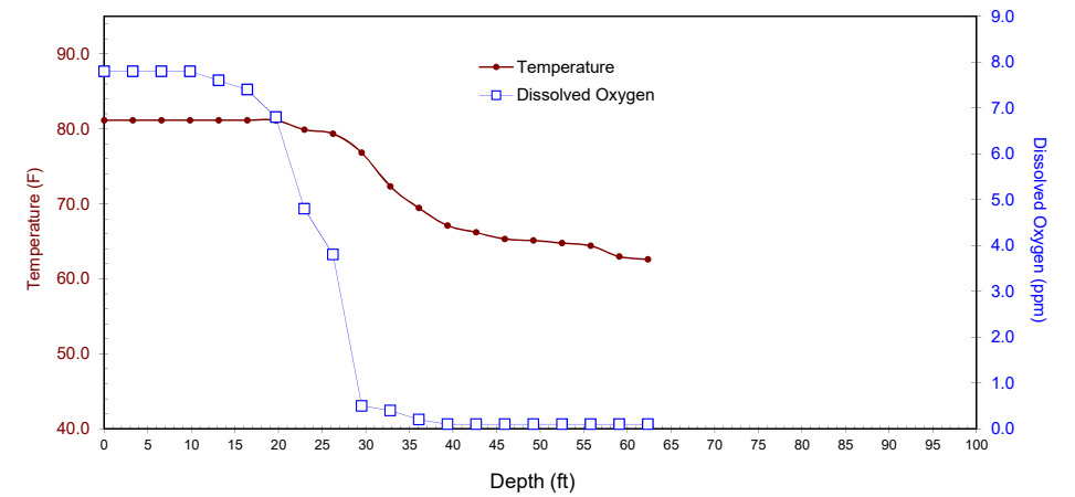
Douglas Reservoir Water Quality at French Broad River Mile 50 - July 11, 2016
